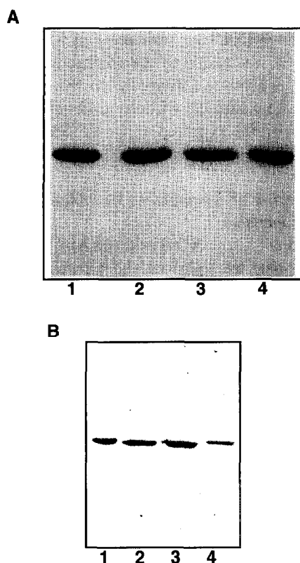
Fig. 2. (A) Coomassie blue-stained SDS-PAGE of purified Drosophila ADH and mutants. (1) 10 \mu g of wild-type ADH from adult flies; 10 \mu l of recombinant ADH purified from E. coli JM105 transformed with (2) pKK223-wild-type ADH; (3) pKK223-Ala 13 Gly mutant and (4) pKK223-Asn 56 Thr mutant. (B) Western blot analysis of purified ADH using mAb LLBE8 against D. lebanonensis ADH. Lanes correspond to the same samples as displayed in (A).
